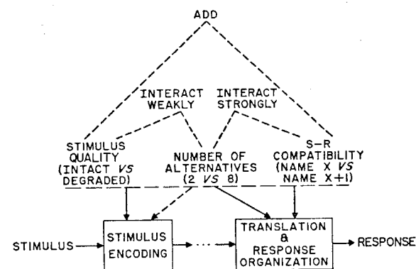
Fig. 10. Relations among factors in exp. V and the inferred stages of processing.
