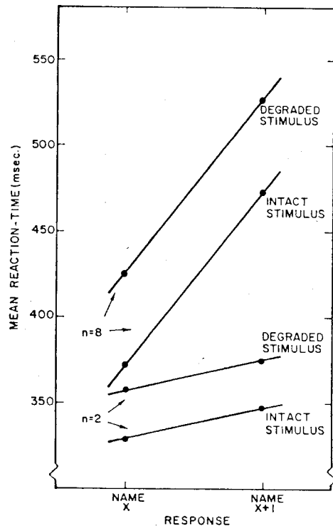
Fig. 8. Mean RTs for the eight conditions in exp. V. On the abscissa are indicated the two levels of compatibility; parameters are number of alternatives ( n ) and stimulus quality. For each value of n is also shown the best-fitting pair of parallel lines, which represent perfect additivity of the effects on mean RT of stimulus quality and compatibility. For n=2 , the mean interaction-contrast is -0.9 msec with an SE of 0.9 msec. For n=8 the mean interaction-contrast is +0.4 msec with an SE of 1.0 msec.
