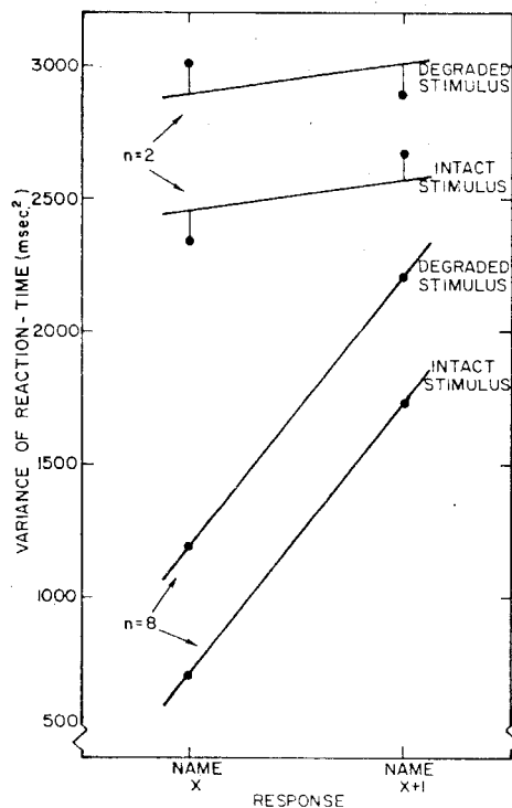
Fig. 11. Average RT-variances for the eight conditions in exp. V. On the abscissa are indicated the two levels of compatibility; parameters are number of alternatives ( n ) and stimulus quality. For each value of n is also shown the best-fitting pair of parallel lines, which represent perfect additivity of the effects on the RT variance of stimulus quality and compatibility. For n=2 the mean interaction-contrast is -111 \text{ msec}^2 with an SE of 45 \text{ msec}^2 . For n=8 the mean interaction-contrast is -7 \text{ msec}^2 with an SE of 41 \text{ msec}^2 .
