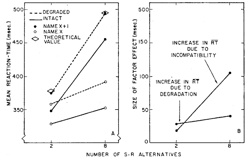
Fig. 9. Interactions between number of alternatives ( n ) and the other factors in exp. V. A: Mean RT to stimuli '1' and '8' as a function of n under four conditions. Theoretical values for the topmost points in each set of four are the values expected from the other three points, combined with the assumption that effects of S-R compatibility and stimulus quality are additive for each value of n . B: Effects of stimulus quality (averaged over compatibility levels) and of compatibility (averaged over quality levels) as a function of n ; derived from values in panel A. Lines would be horizontal if these factors did not interact with n .
