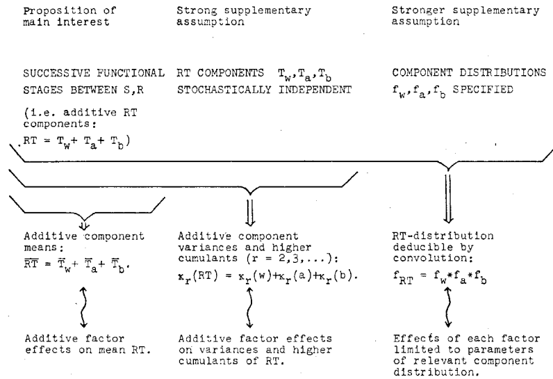
Fig. 1. Three types of assumption in the decomposition of RT, and their implications. Wavy arrows show loose implications (see section 3.1); statements in bottom row apply only to experimental factors that influence no stages in common.
