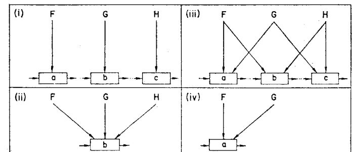
Fig. 3. Some possible arrangements of factors and stages.
