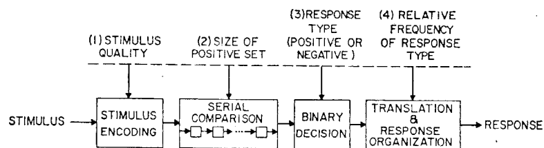
Fig. 6. Processing stages in binary classification. Above the broken line are shown the four factors examined. Below the line is shown the analysis of RT inferred from additive relations between factor pairs 1&2, 1&3, 2&3, 2&4, and 3&4, the linear effect of factor 2, and other considerations described in the text. The quality of the test stimulus influences the duration of an encoding stage in which a stimulus representation is formed. This representation is then used in a serial-comparison stage, whose duration depends linearly on size of positive set; in each of its substages the representation is compared to a memory representation of one member of the set. In the third stage a binary decision is made that depends on whether a match has occurred during the serial-comparison stage that precedes it; its mean duration is greater for negative than for positive decisions. The selection of a response based on the decision is accomplished in the final stage whose duration depends on the relative frequency with which a response of that type is required.
